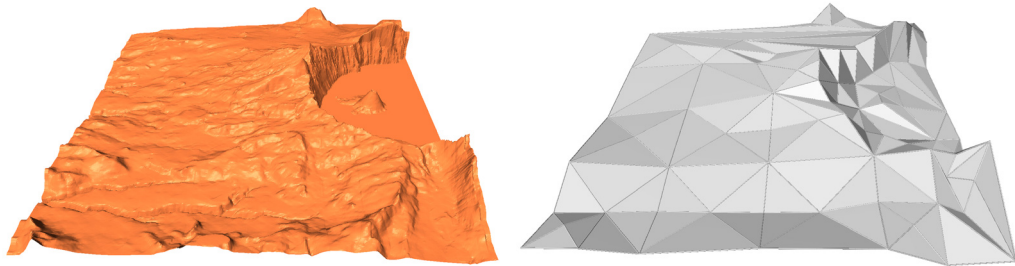
Figure 2.6: Bivariate approximation of Crater Lake data set. Left image shows the original data set F(x, y) . Right image shows the approximation A(x, y) having 93 knots and 159 triangles. The approximation has an error of 8.62.
