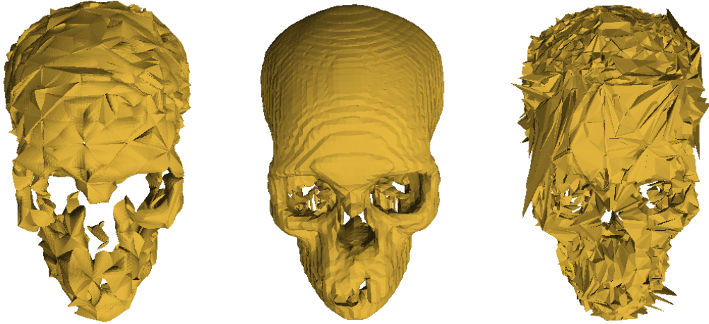
Figure 3.8: Comparison between quadratic approximation (left) and linear approximation (right). Original skull is shown in the center image. The quadratic approximation uses 7487 knots and 5348 elements. The linear approximation uses 14667 knots and 78530 elements. Image-space errors are 8.12% and 8.33% for the isosurface images from the quadratic and linear approximation, respectively.
