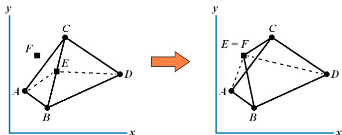
Figure 2.11: Example of malformed triangles when the midpoint E of the longest edge (formed by B and C ) is snapped to a knot location F outside of the domain of the triangle(s) being refined.
