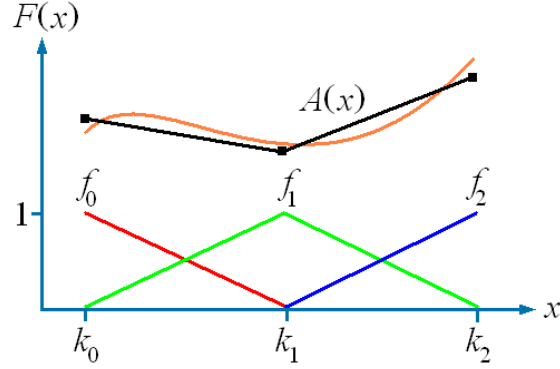
Figure 2.2: Best-approximation example. Orange curve shows the original function F(x) . Black line segments show the linear spline approximation A(x) . Basis functions f_0 , f_1 , and f_2 are shown for knot locations k_0 , k_1 , and k_2 , respectively.
