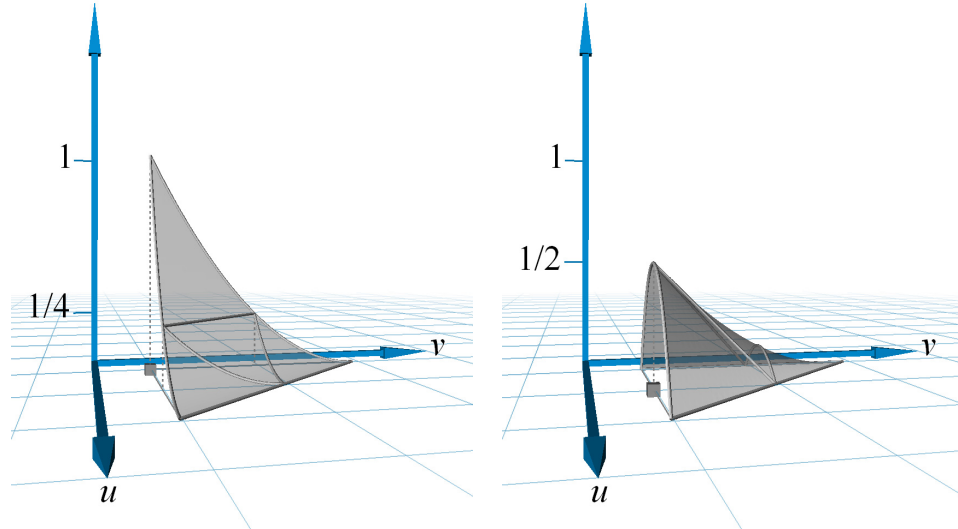
Figure 3.3: Bivariate quadratic basis (or “shape”) functions. Left image shows the basis function B_{0,0}^2(u,v) = (1-u-v)^2 associated with corner knot located at \mathbf{u}_{0,0} = (0,0)^T . Right image shows the basis function B_{1,0}^2(u,v) = 2(1-u-v)u associated with edge knot located at \mathbf{u}_{1,0} = (\frac{1}{2}, 0)^T .
