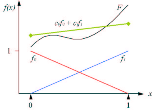
Fig. 1. Basis functions f_i , function F to be approximated, and approximation f(x) = c_0 f_0 + c_1 f_1
