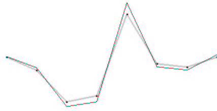
Fig. 7. Demonstration of effect of over- and under-shoots. The lighter polygon shows the original function; the darker polygon shows the approximation
